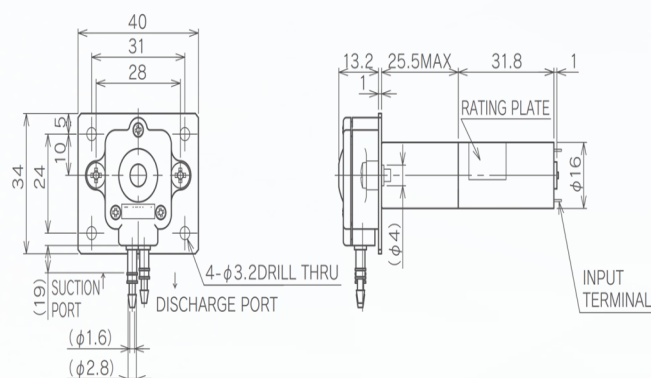
Outline drawing
