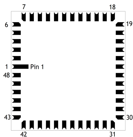
Figure 5. Package Drawing Bottom View
