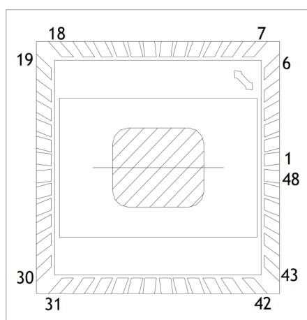
Figure 4. Package Drawing Top View
