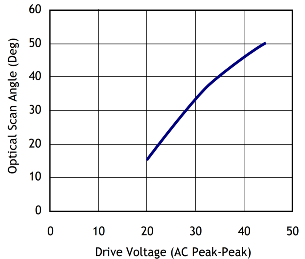
Figure 2. Typical Scan Angle vs. Drive Voltage with Constant Driving Frequency
