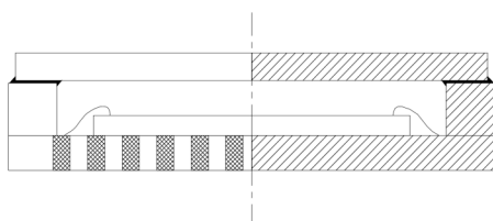
Figure 6. Package Drawing Side View
