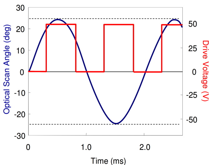
Figure 3. Typical Scan Trajectory Versus Drive Signal
